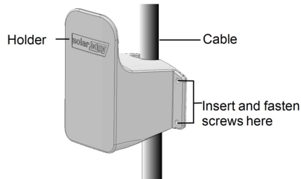
Figure 2: Cable connection
